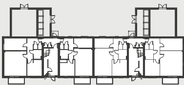
Ground Floor
